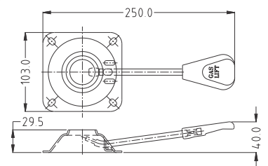
EPS-05 Lever for seat height adjustment
