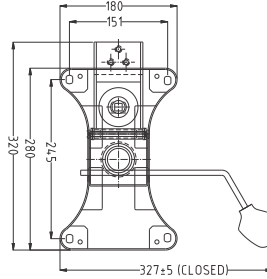
EPS-02 Lever for seat height adjustment
